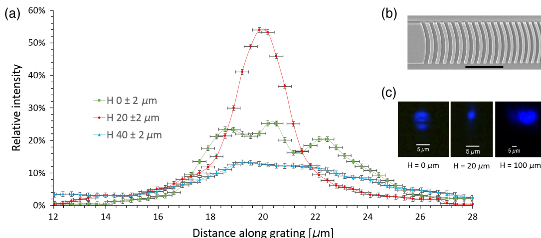
Fig. 7 (a) Relative intensity of the output spot of the probe focusing grating. The grating shown is been designed for blue light (450 nm), with a focusing height of 20 \mu\text{m} above the device plane. The intensity is plotted as function of a line along the focusing grating direction. The three curves show the image intensity recorded at different heights with respect to the grating's plane ( h = 0 means the camera focus lies on the grating and h = 10 means the camera focus is 10 \mu\text{m} above the grating plane); error bars for the vertical axis correspond to noise (in plane scattered light). Error bars on the horizontal axis correspond to the pixel size. (b) SEM image of the probe focusing grating. (c) Output spot images at different camera heights. Left: CCD camera focused on grating plane. Center: CCD camera focused 20 \mu\text{m} above the grating plane (the focal plane). Right: CCD camera focused 100 \mu\text{m} above the grating plane; after the focusing point, the beam broadens.
