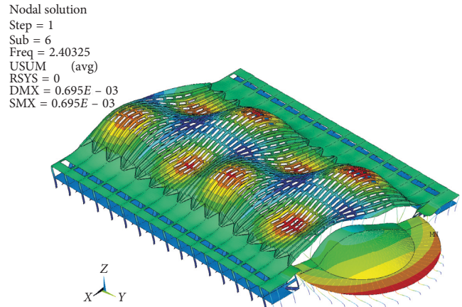
FIGURE 13: Mode 6 of Hall B in its damaged configuration (aspe view).
