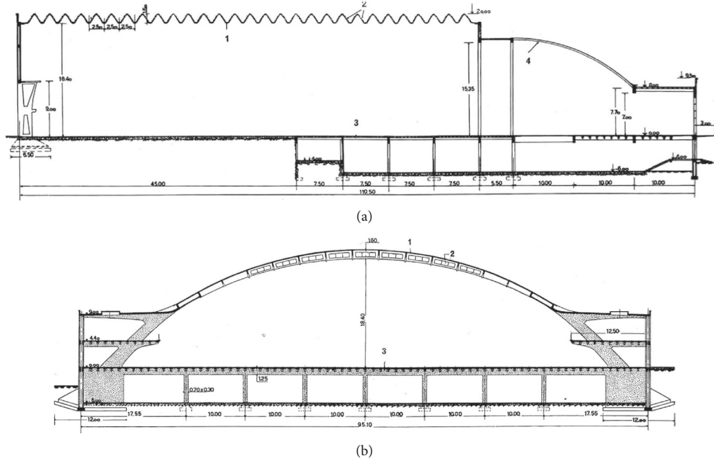
FIGURE 3: Sections of Hall B [34].
