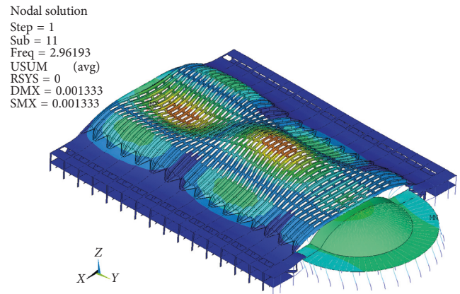
FIGURE 14: Mode 11 of Hall B in its damaged configuration (aspe view).
