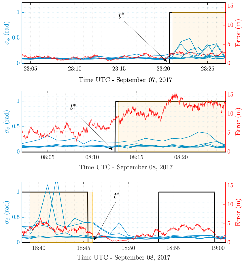
Figure 10. Comparison of \sigma_\phi index for visible satellites (light blue), position solution error (orange), and clustering-derived detection (black).
