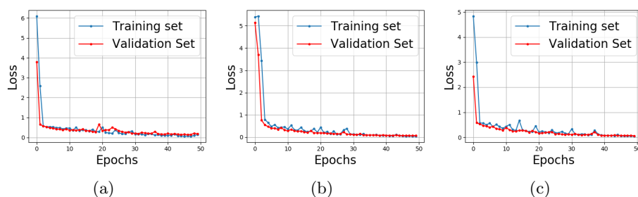
Fig. 2. Loss functions of CNN models using different encodings: 2(a) ordinal encoding, 2(b) standard one-hot encoding and 2(c) Bulka's encoding.
