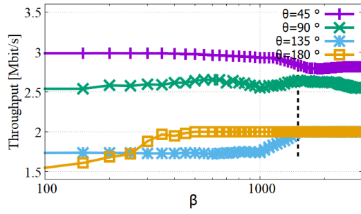
Fig. 5. Throughput in function of \beta under scenario C.
