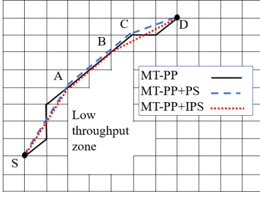
Fig. 2. An example showing the difference between our smoothing method A*IPS with respect to A*PS.
