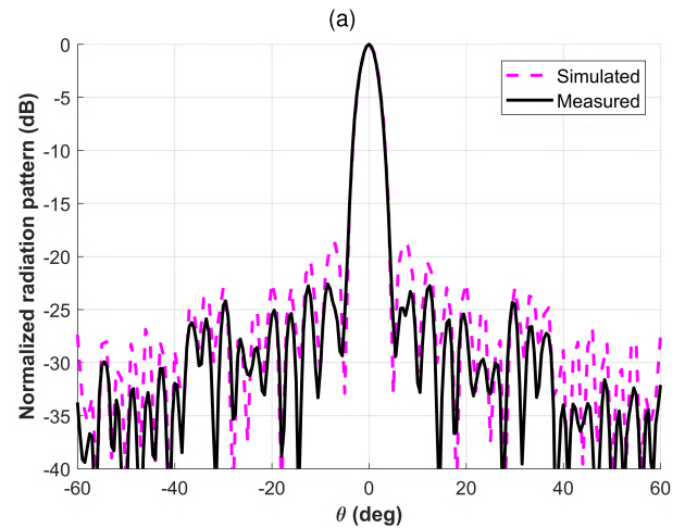
FIGURE 18. Measured and simulated co-polar radiation patterns of the 3D-printed TA prototype (TA4), at 30 GHz: (a) H-plane; (b) E-plane.
