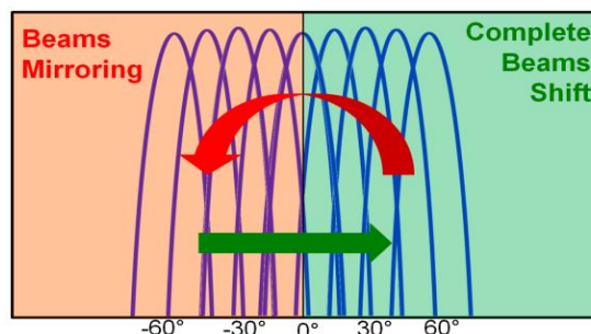
Fig. 1. Combination of “Complete Beam Shifting” and “Beam Mirroring” for scanning range extension of Rotman lenses.
