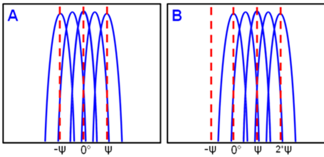
Fig. 3. Working principle of the complete beam shifting effect. In picture A) the beams are related to the antenna array only, while in B) the beams are shifted towards positive scan angles by applying the beam shifting.
