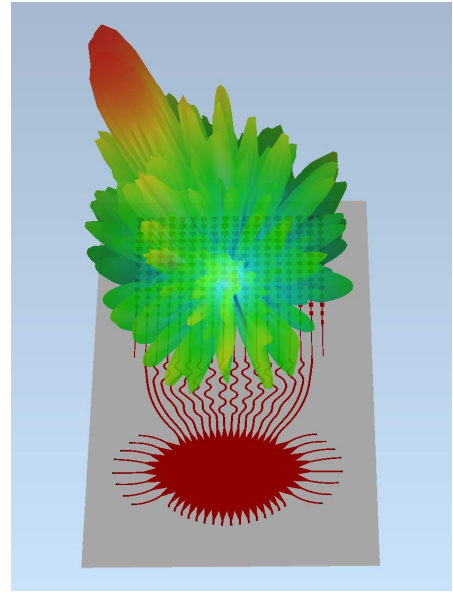
Fig. 1. Standard approach for antenna array beamforming employing Rotman Lens.
