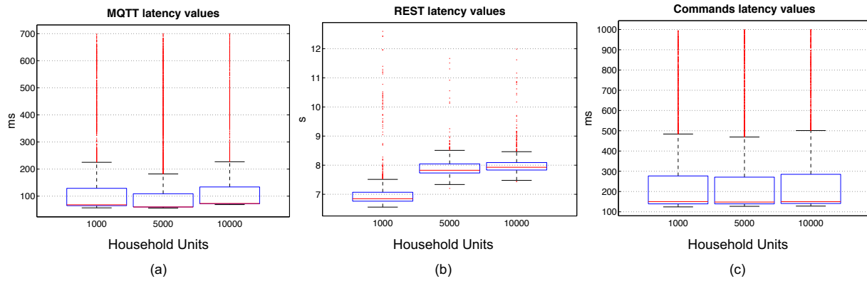
Fig. 11. Transmission latency at different Household Units: (a) MQTT, (b) REST, (c) Commands.
