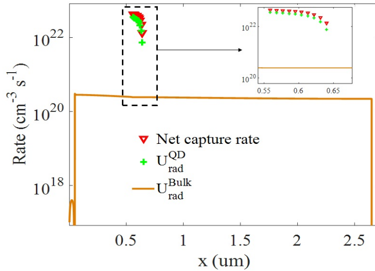
Fig. 2.8 Bulk radiative recombination rate along with the equivalent volume recombination and net capture rates of QD states at open circuit condition.
