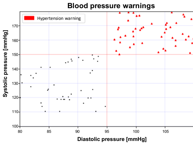
Fig. 4. Blood pressure and Hypertension warnings.
