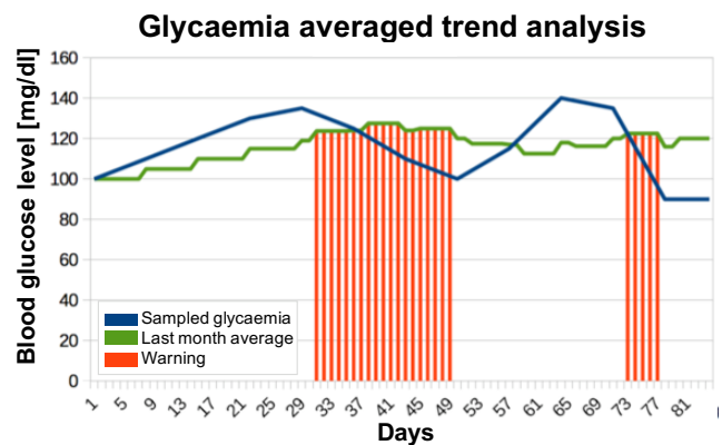
Fig. 11. Warnings triggered by Glycaemia averaged trend rule .
