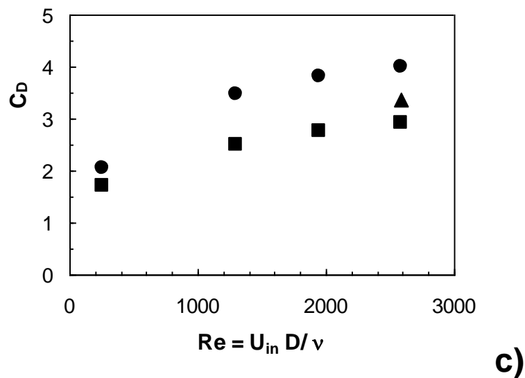
Figure 9. Mushroom valve. a) Required inlet pressure (for a condenser pressure = 4 Pa) as a function of the sublimation rate in the industrial scale freeze-dryer chamber, for different values of the disk valve distance (in mm). b) Force on the valve disk, as a function of the sublimation rate, for different valve disk distances (in mm). c) Drag coefficient vs. Reynolds number for the disk of the mushroom valve.
