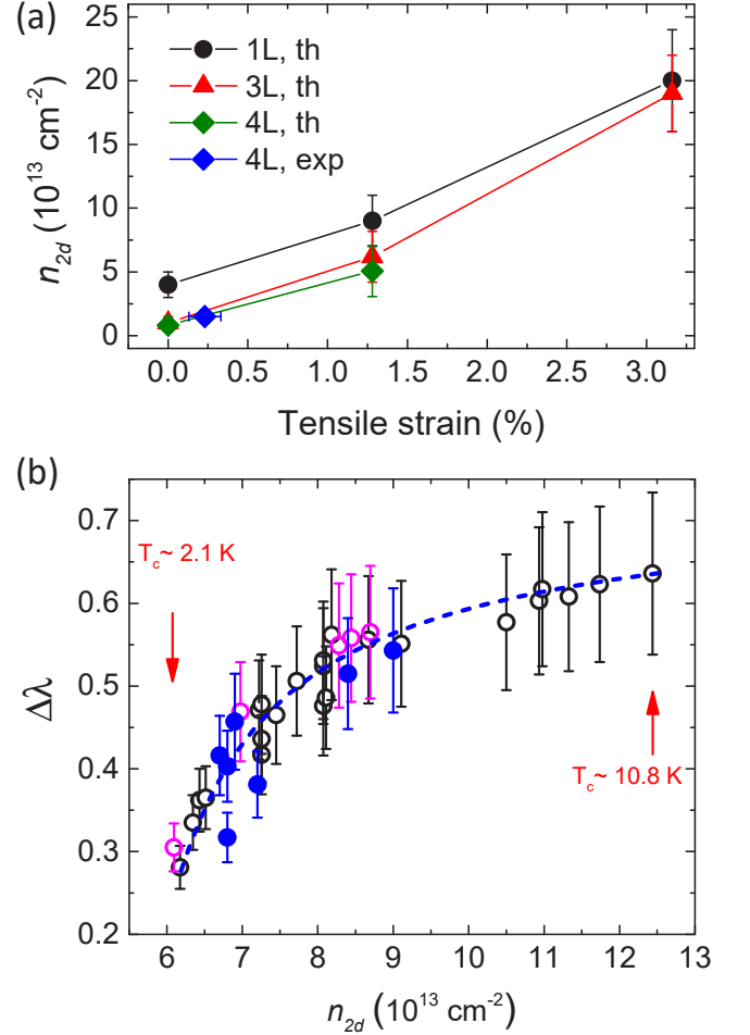
FIG. 7. a) Surface carrier densities required to cross the Q 1 sub-band in FL-MoS 2 as a function of tensile strain. Theoretical values for 1L (black dots and line) and 3L (red triangle and line) from Ref. 46; values for 4L (green diamonds and line) are by linear extrapolation. Blue diamond is the present experiment. b) EPC enhancement due to the crossing of the Q 2 sub-band, Δλ, as a function of n 2d , assuming ω ln = 230 ± 30K and μ* = 0.13 18 . Filled blue circles are our experiments. Black and magenta open circles from Refs. 23,31. The blue dashed line is a guide to the eye.
