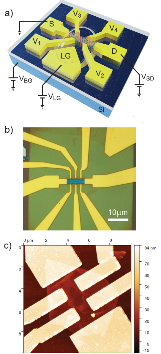
FIG. 2. a) Hall bar FL-MoS 2 flake with voltage probes ( V_i ), source (S), drain (D) and liquid-gate (LG) electrodes. A ionic liquid droplet covers the flake and part of the LG electrode. The sample is biased with a source-drain voltage ( V_{SD} ) and dual gate control is enabled by a voltage applied on the liquid gate ( V_{LG} ) and on the solid back gate ( V_{BG} ). b) Optical image of Hall bar with six voltage probes. The LG electrode is on the upper-right corner. c) AFM scan of the MoS 2 Hall bar after ionic liquid removal.
