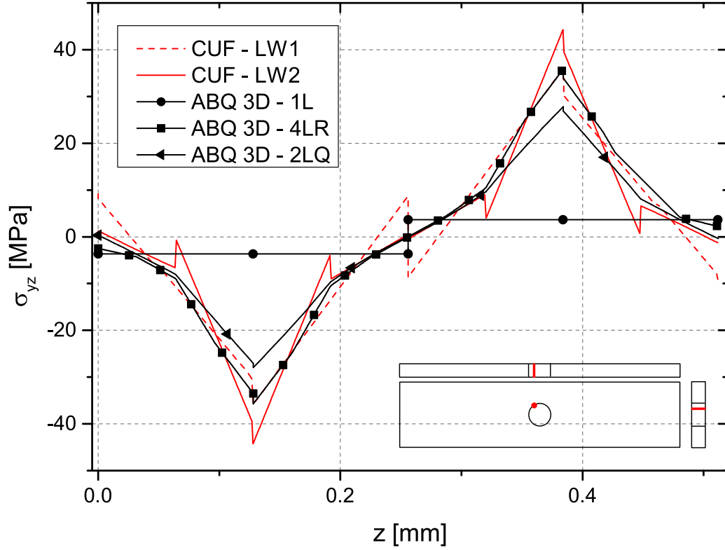
Figure 21: Transverse shear stress distribution \sigma_{yz} through the thickness of [0/90]_s notched laminate under an applied displacement of 0.125 mm, x = 17.04 , y = 68
