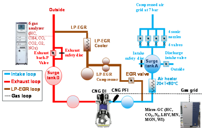
Figure 2. Single-cylinder engine installation on the test bench.
