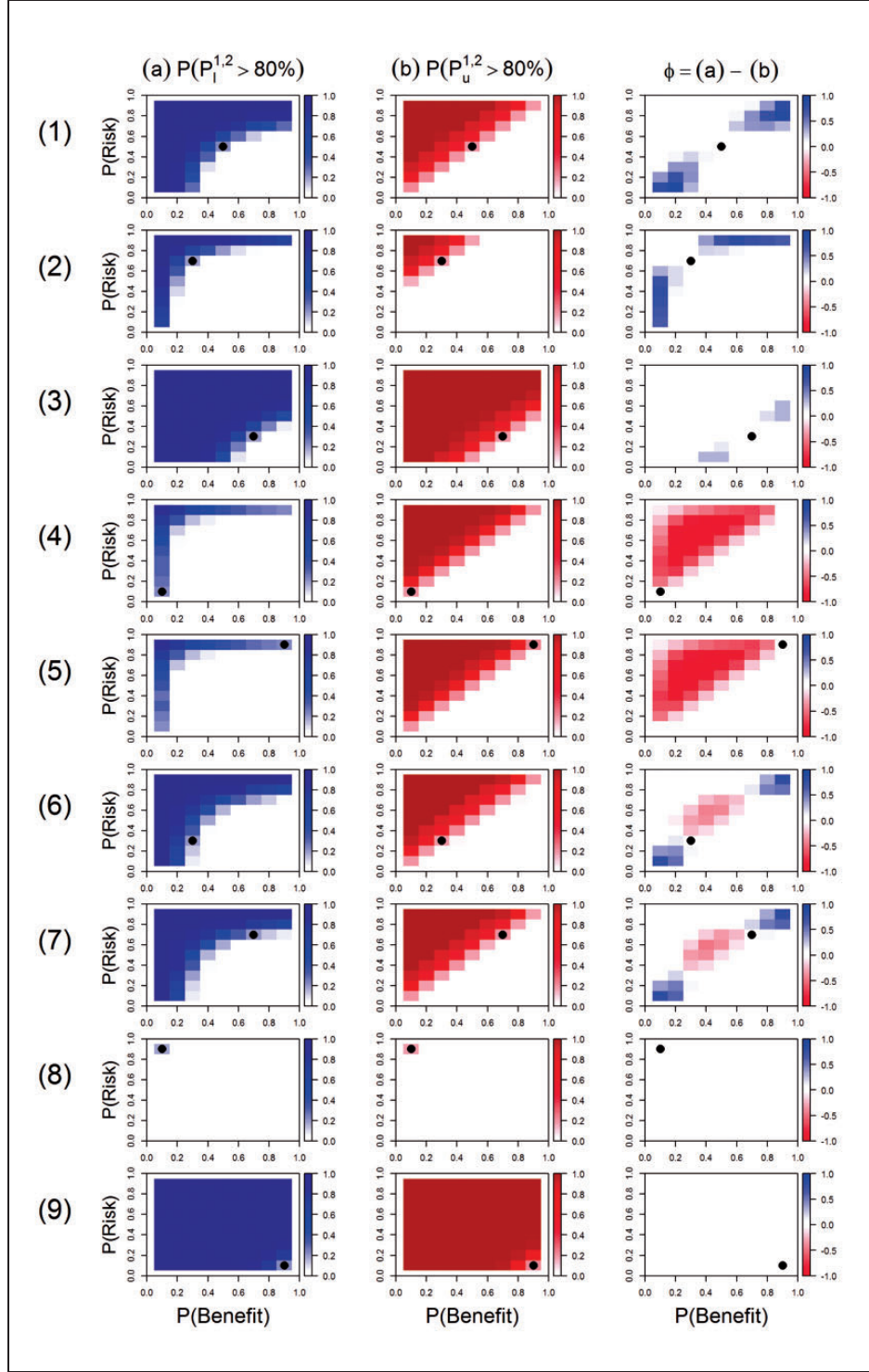
Figure 4. Results of MCDA and SLoS performances in all simulation scenarios for two equally important criteria ( w_j = \tilde{w}_j = 0.5 for j = 1, 2 ). \bullet = T_I . Left panel: P[P^{1,2}_l > 0.8] . Middle panel: P[P^{1,2}_u > 0.8] . Right panel: \Phi = P[P^{1,2}_l > 0.8] - P[P^{1,2}_u > 0.8] , for which blue cells (resp., red cells) indicate that SLoS recommends T_I more often (resp., less often) than MCDA.
