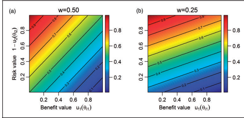
Figure 1. Left panel: contours of equal linear loss score \bar{u}(\theta_{i1}, \theta_{i2}, w=0.5) . Right panel: contours of equal linear loss score \bar{u}(\theta_{i1}, \theta_{i2}, w=0.25) .
