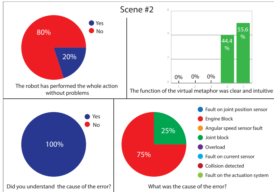
Fig. 9. Scene 2 results.
