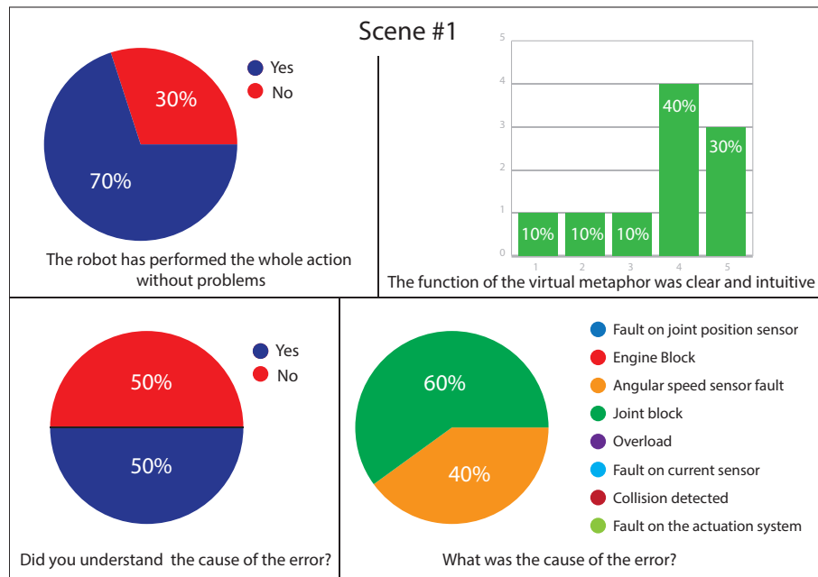
Fig. 8. Scene 1 results.
