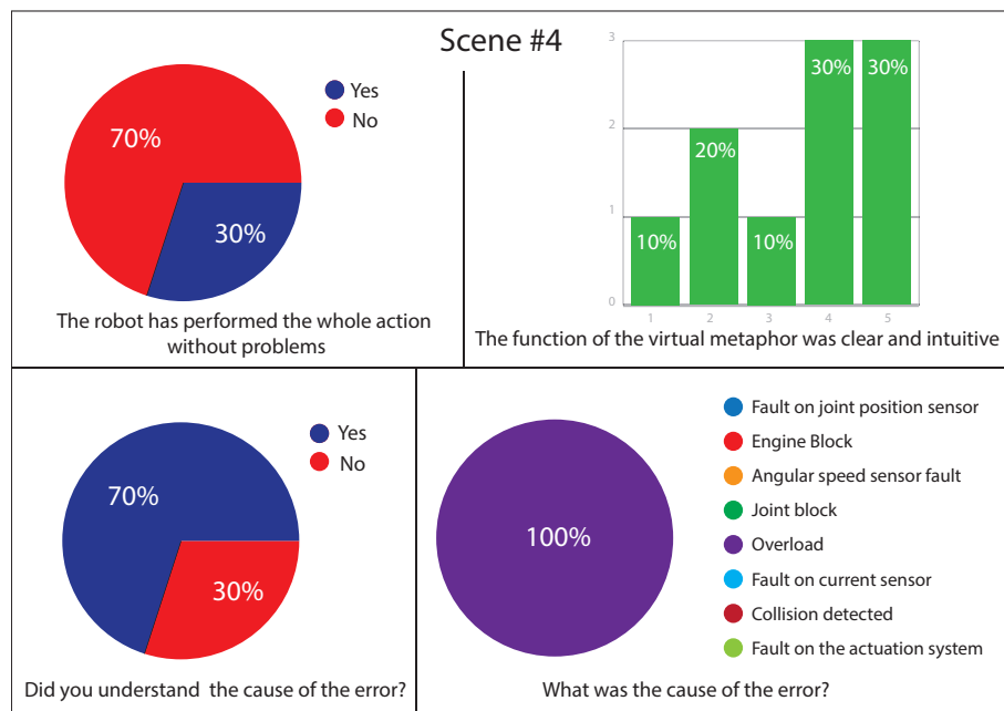
Fig. 12. Scene 4 results
