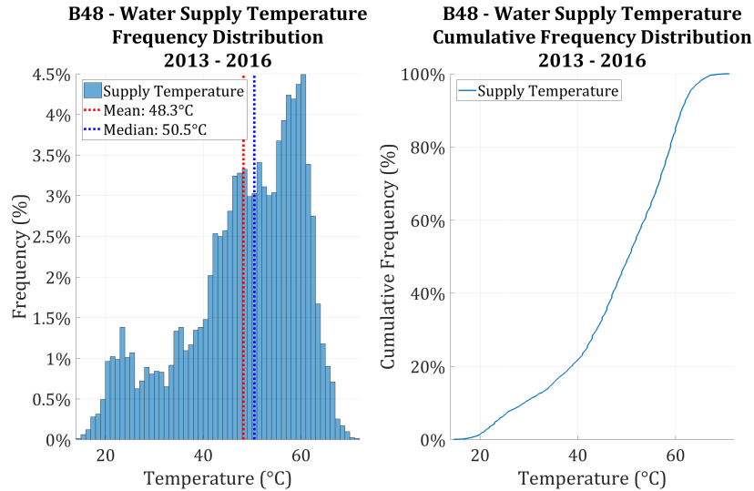
Figure 7: B48 - Water supply temperature relative and cumulative relative distribution.
