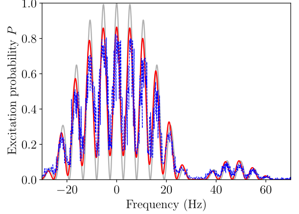
FIG. 5 Experimental Ramsey spectrum (blue dashed line) for \tau = 30 \text{ ms} \frac{\pi}{2} pulses and T = 150 \text{ ms} with an atom number of \sim 1500 , which corresponds to an average number of 1.5 \sim 3 atoms per lattice site. To increase atomic interactions, the trap depth is set to a large value of 650E_r . Gray line indicates the theoretical spectrum without atomic interactions. Red line includes interactions with \bar{W} = 2\pi \times 1.6 \text{ Hz} obtained from experimental data by the asymmetry-based measurement.
