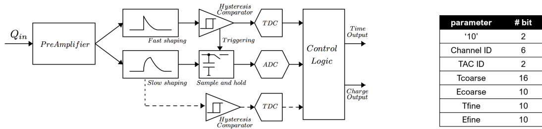
Figure 1: Block diagram of one channel (left) and one output event word (right).
