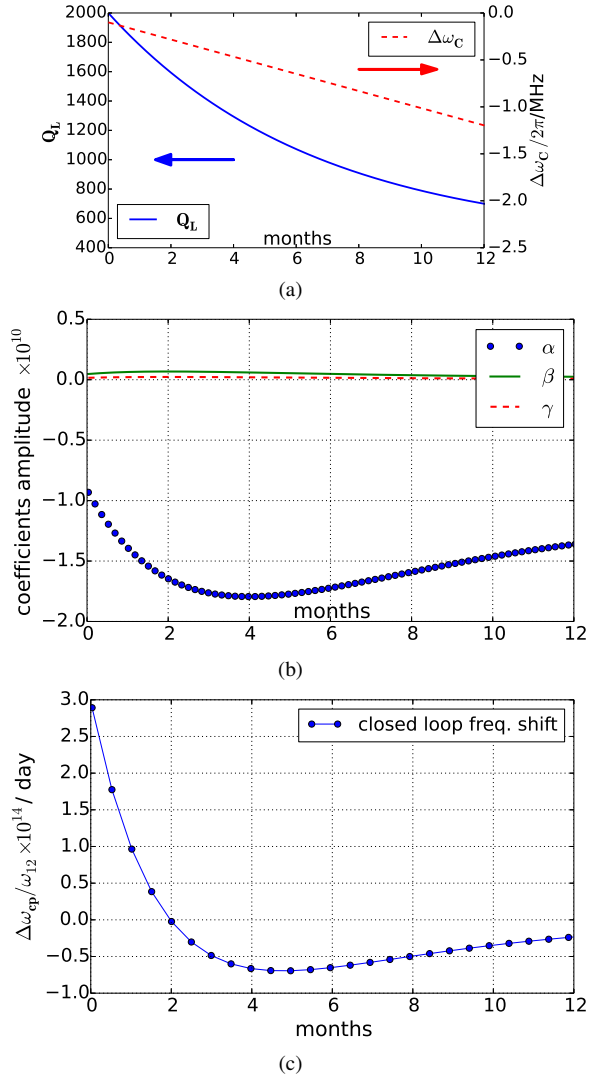
Figure 6. (a) Detuning and Q -factor evolutions during a one-year period as assumed in the model calculations. (b) Sensibility coefficients of eq. (7) during the same period. (c) Daily frequency variation, with pulse area actively stabilized at \pi/2 , due to a change in the cavity pulling shift (eq. (9)) as Q_L and \Delta \omega_C change during one year.
