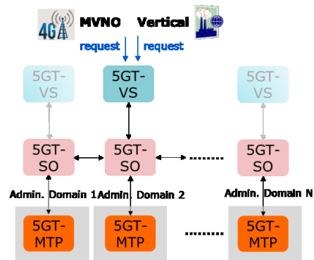
Figure 1: The 5G-TRANSFORMER concept
