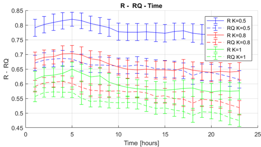
Figure 10. Resilience indices R and R_Q for three K_I values (pipe material).
