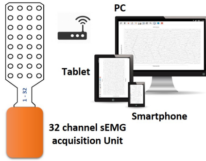
Fig. 1. System architecture. The developed system is composed by one sensor unit that conditions, samples, and transmits up to 32 monopolar sEMG and 3 auxiliary signals sampled at 2048 ksps with 16 bit resolution and one mobile device (notebook, tablet or smartphone) that receives wirelessly the sampled signals. The transmitter and the receiver are connected through a wireless access point.
