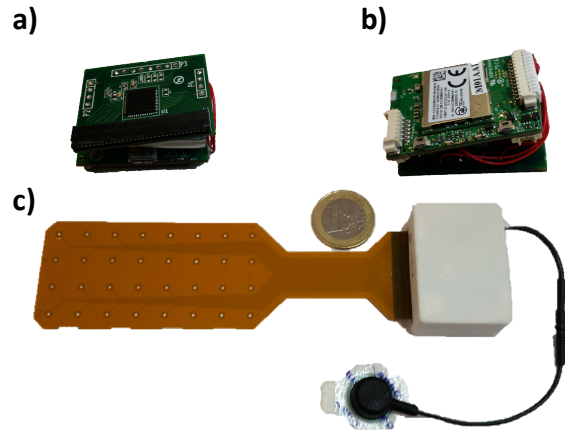
Fig. 3. The sensor unit prototype is composed by two interconnected PCBs mounting the a) biosignal acquisition unit and b) the wireless MCU, the power supply and the battery charging circuit. The battery is mounted between the two interconnected PCBs. c) The system prototype was encapsulated in a 3D printed case and connected to a flexible kapton matrix (8x4 electrodes with 10 mm interelectrode distance). The overall system's dimensions are 37 mm x 33 mm x 20 mm.
