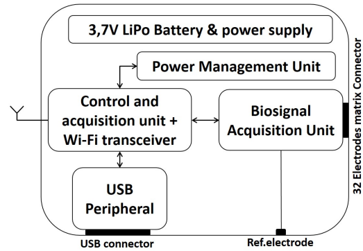
Fig. 2. Block diagram of the Sensor Unit. The control and acquisition unit is based on a wireless Microcontroller (Texas Instruments CC3200) It communicates with the Intan RHD2132 biosignal acquisition system (through a SPI bus) with the USB Peripheral interface and provides to send wirelessly the sampled data. The Biosignal Acquisition unit provides amplification (192 V/V), conditioning (10Hz-500Hz) and quantization of 32 sEMG signals plus 3 auxiliary signals. The Power supply unit provides a regulated 3.3V power supply while and the Power Management Unit allows to charge the system through the USB connector. The USB peripheral is also used for debug purposes.
