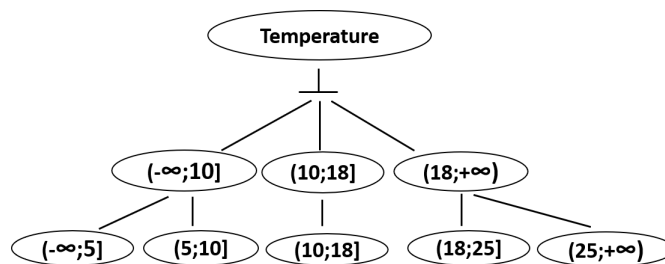
Figure 2. Example of a generalization tree for the temperature attribute.
