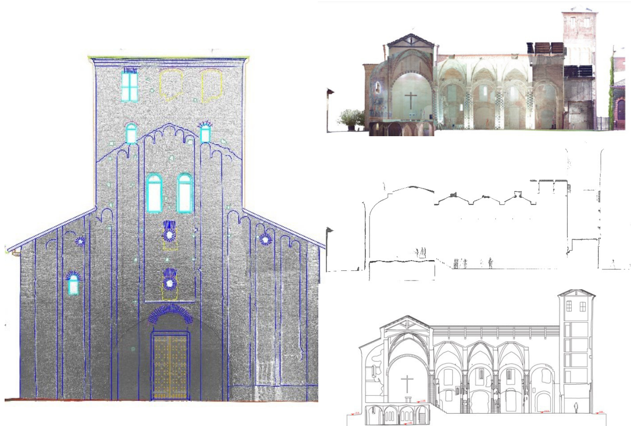
Fig. 4 – Elevation (left) and section vector-based extraction (right – Top: point cloud – Middle: section line – Bottom: complete section vector-dataset)
