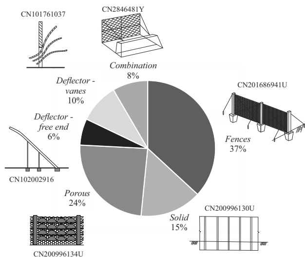
Fig. (4). Windblown sand barriers classification and distribution.
