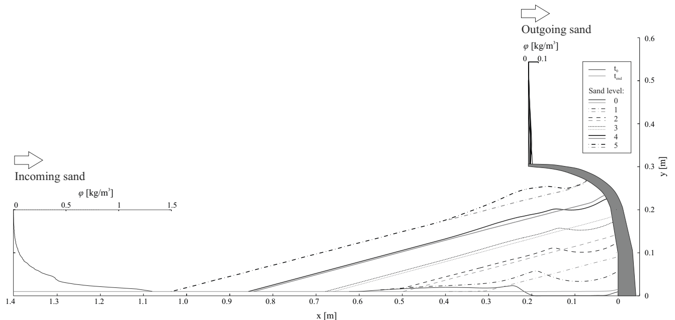
Fig. (12). Sand accumulation profiles against S4S barrier and incoming and outgoing sand concentration \phi .
