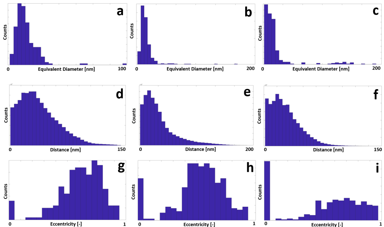
Figure 3 Geometrical statistics extracted from the FESEM images of Figure 2, with varying concentration of \text{AgNO}_3 : 5 (left column), 20 (middle column), and 50 phr (right column), showing their properties: the equivalent diameter (upper row), the inter-particle distance (middle row) and the eccentricity (bottom row).
