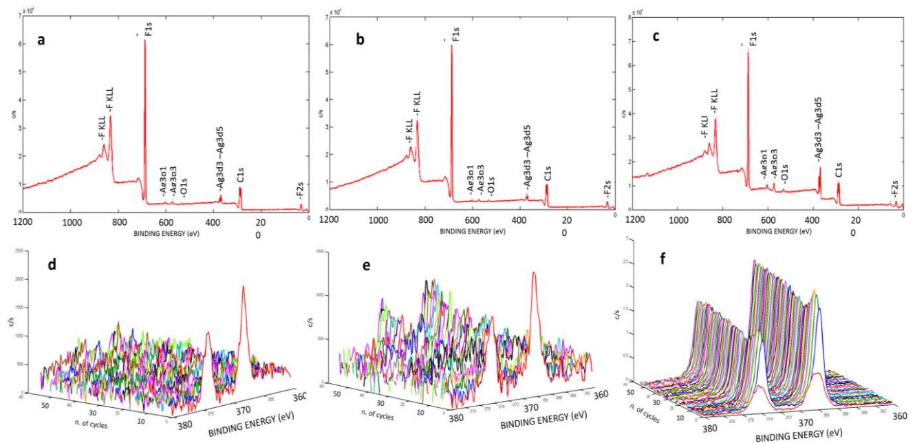
Figure 4 XPS survey spectra (upper row) for the 5 (a), 20 (b) and 50 (c) AgNO 3 samples. Ag3d (lower row) HR spectra collected during the depth profile acquisition for all the the 5 (d), 20 (e) and 50 (f) AgNO 3 samples.
