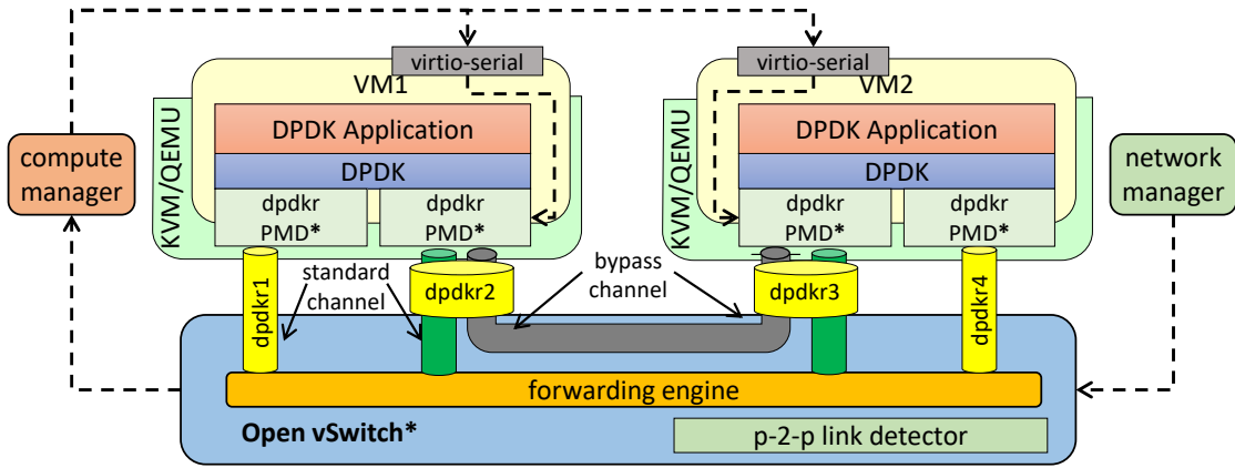
Figure 10: Implementing direct channels between VMs in OvS. Components marked with '*' have been modified to support transparent inter-SF communication.
