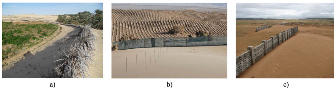
Fig. 23. Fences with smeared porosity: a) traditional fence protecting a palm plantation (explicit publishing permission from the owner of the photos: Nour Boulghobra); b) nylon net fence (reprinted from: Liu et al., 2014 , with the permission to reuse under a Creative Commons Attribution License). Fences with localized porosity: c) concrete fence (reprinted from: Zhang et al., 2010b , with the permission from Elsevier).
