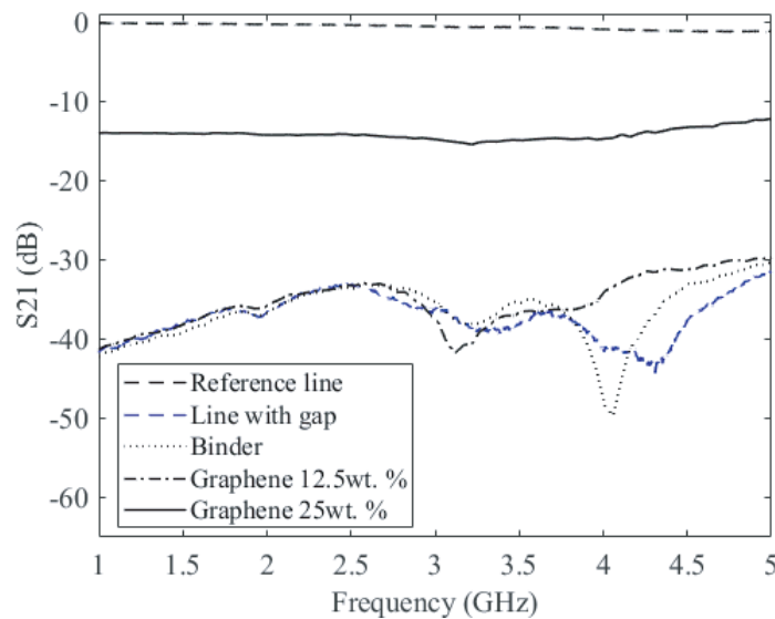
Figure 2. Measurement of the transmission coefficient magnitude of the reference line and of the microstrip line with gap for various graphene-loading compositions.
