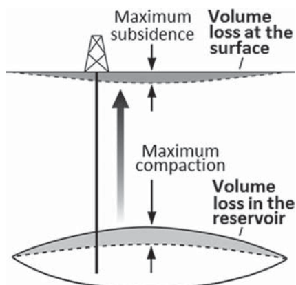
Fig. 7. Compaction and subsidence (adapted from Fjær et al. , 2008). Compattazione e subsidenza (modificata da Fjær et al. , 2008).
