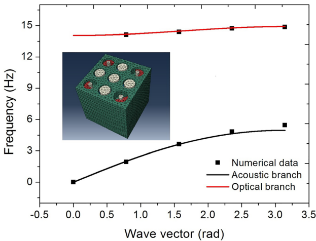
FIG. 3. Dispersion curve computed from the dispersion relationship [Eq. (1); solid lines] for periodic mass-in-mass systems ( L=0.2 \text{ m} , m_i=317 \text{ kg} , m_e=245 \text{ kg} , k_e=155 \times 10^3 \text{ N/m} , and k_i=1080 \times 10^3 \text{ N/m} ) and three-dimensional finite-element simulations (squares). The inset shows the three-dimensional finite-element discretization scheme used for the CF in which four plates are separated by an ideal disconnection plane.
