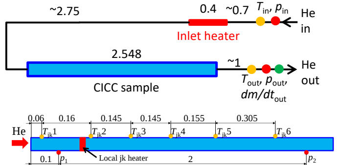
Fig. 3. Sketch of the location of (a) inlet heater, p , T and dm/dt facility sensors, and (b) sensors installed on the sample (all quotes are in m). The inlet and outlet pipes diameter is 6 mm (inner) × 8 mm (outer).
