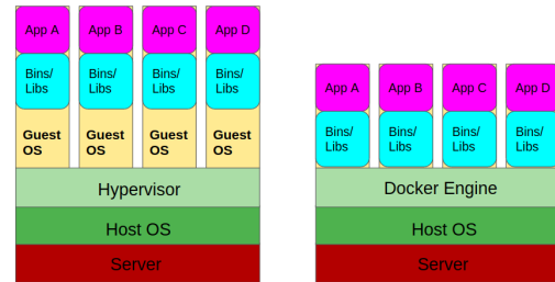
Fig. 1. High-level architecture of virtual machine-based virtualization (left) and container-based virtualization (right).
