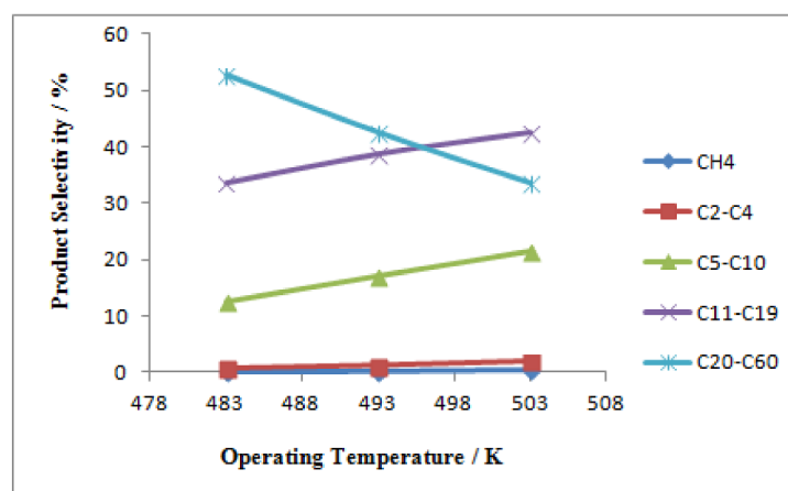
Figure 9. Influence of operating temperature on product selectivity; D_t = 0.1 m, H = 2.5 m, V_f = 3.5 m³/h, P = 20 bar, \varepsilon_{cat} = 0.34 .
