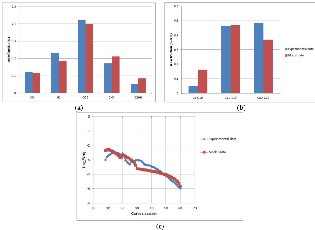
Figure 7. The comparison of the predicted model with experimental data at change load conditions (volumetric gas flow rate 7.5 \text{ m}^3/\text{h} , T = 503 \text{ K} , \varepsilon_{\text{cat}} = 0.34 , P = 20 \text{ bar} ): (a) off-gas molar fractions; (b) FT products (naphtha, diesel, wax); (c) ASF distribution.
