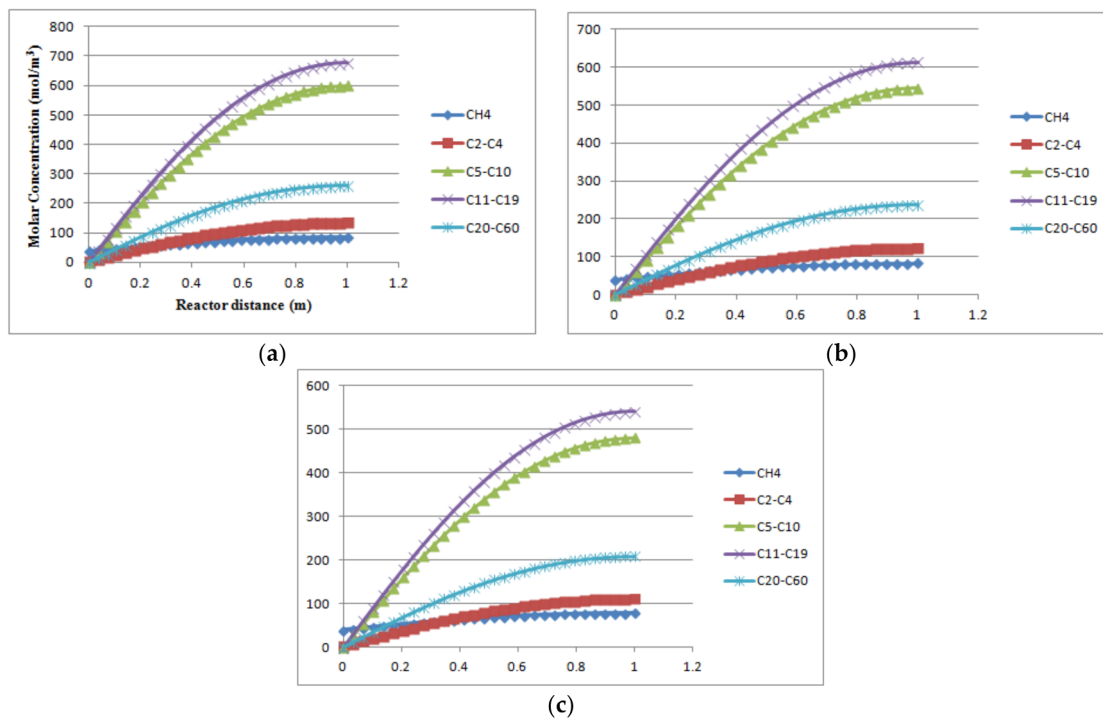
Figure 13. The molar concentration of the FT products along the reactor bed at three load conditions: (a) T = 503\text{ K} , P = 20\text{ bar} , V_f = 3.5\text{ m}^3/\text{h} ; (b) T = 503\text{ K} , P = 20\text{ bar} , V_f = 5\text{ m}^3/\text{h} ; (c) T = 503\text{ K} , P = 20\text{ bar} , V_f = 7.5\text{ m}^3/\text{h} .
