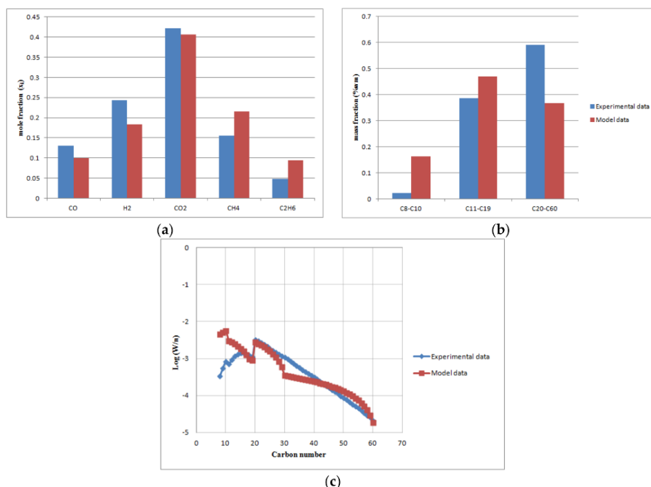
Figure 5. The comparison of the predicted model with experimental data at base load conditions (volumetric gas flow rate 5 m^3/h , T = 503 K, \varepsilon_{cat} = 0.34 , P = 20 bar): (a) off-gas molar fractions; (b) FT products (naphtha, diesel, wax); (c) ASF distribution.
