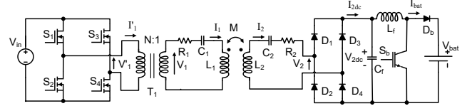
Fig. 4. Power circuit configuration of system B
