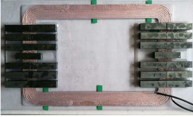
Fig. 5. Structure of the receiver coil
