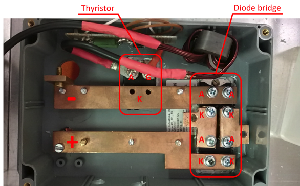
Fig. 7. Top view of the implemented system where the filter capacitors are not mounted. The bus bar structure is visible together with the mounting positions of the thyristor T and the diode bridge.
