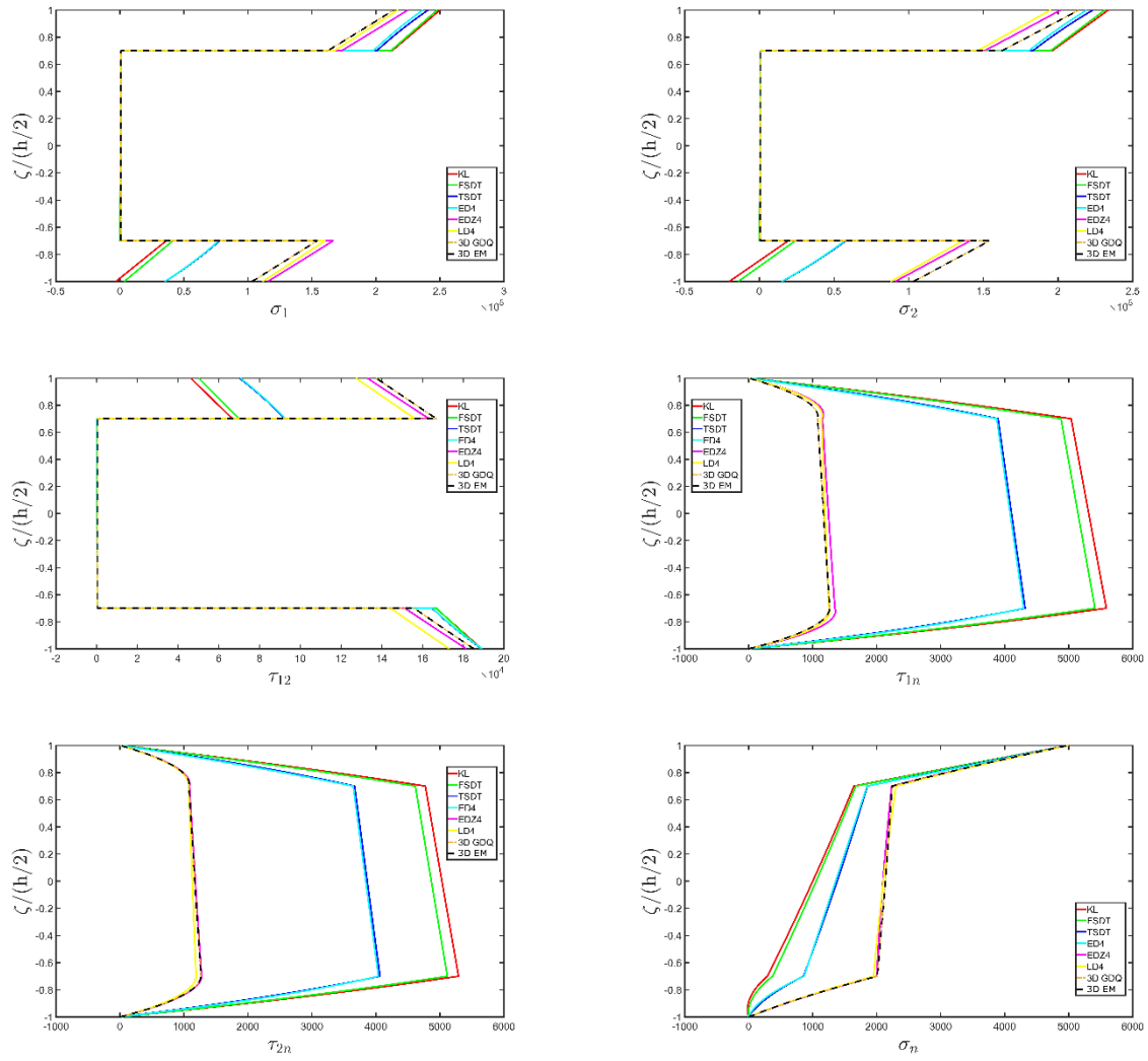
Figure 22. Through-the-thickness variation of stress components [Pa] for a SSSS spherical panel ( R/h=20 ) made of three layers (Titanium / Foam / Titanium) with h_1 = h_3 = 0.15h , h_2 = 0.7h at the point P = (0.25(\alpha_1^1 - \alpha_1^0), 0.25(\alpha_2^1 - \alpha_2^0)) subjected to a normal sinusoidal load q_3^{(+)} = 10000 Pa with n=1, m=1 on the top surface. Comparison between different structural theories.
