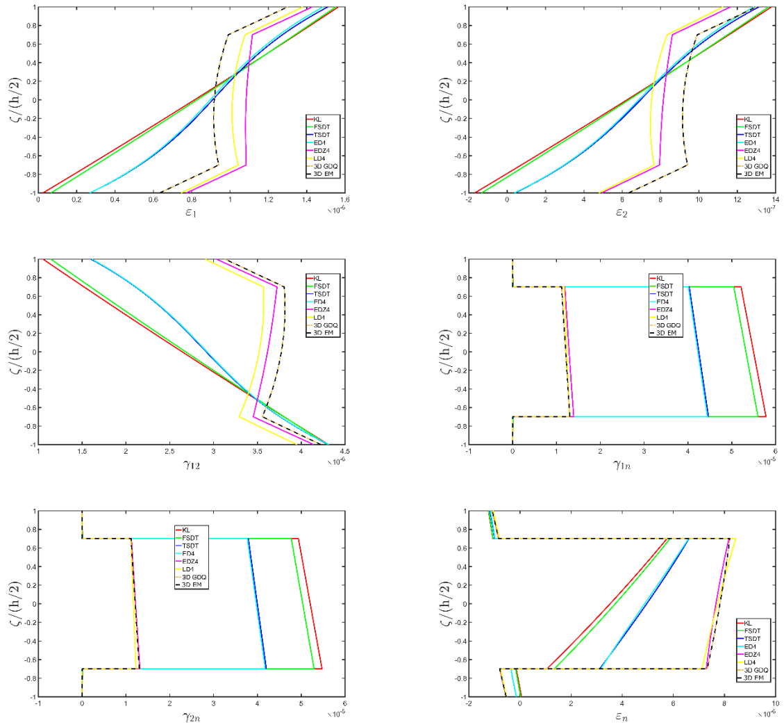
Figure 21. Through-the-thickness variation of strain components for a SSSS spherical panel ( R/h=20 ) made of three layers (Titanium / Foam / Titanium) with h_1 = h_3 = 0.15h , h_2 = 0.7h at the point P = (0.25(\alpha_1^1 - \alpha_1^0), 0.25(\alpha_2^1 - \alpha_2^0)) subjected to a normal sinusoidal load q_3^{(+)} = 10000\text{Pa} with n=1, m=1 on the top surface. Comparison between different structural theories.
