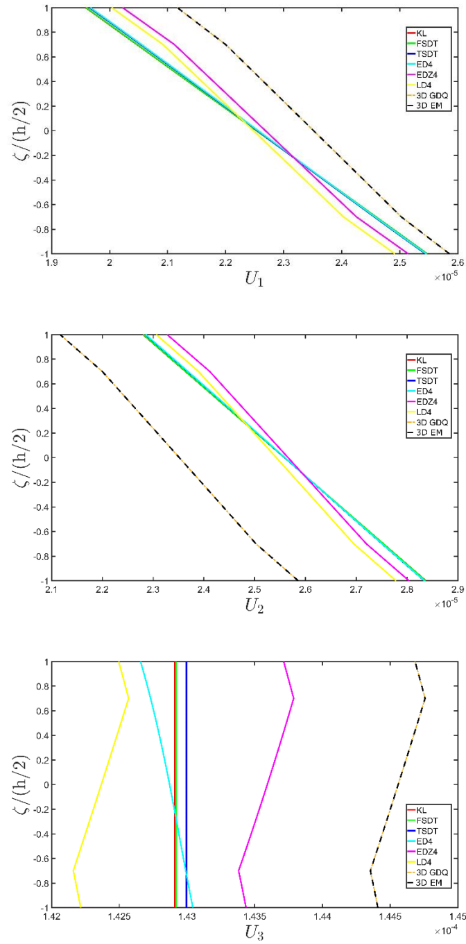
Figure 26. Through-the-thickness variation of displacement components [m] for a SSSS spherical panel ( R/h=100 ) made of three layers (Titanium/Foam/Titanium) with h_1 = h_3 = 0.15h , h_2 = 0.7h at the point P = (0.25(\alpha_1^1 - \alpha_1^0), 0.25(\alpha_2^1 - \alpha_2^0)) subjected to a normal sinusoidal load q_3^{(+)} = 10000\text{Pa} with n=1, m=1 on the top surface. Comparison between different structural theories.
