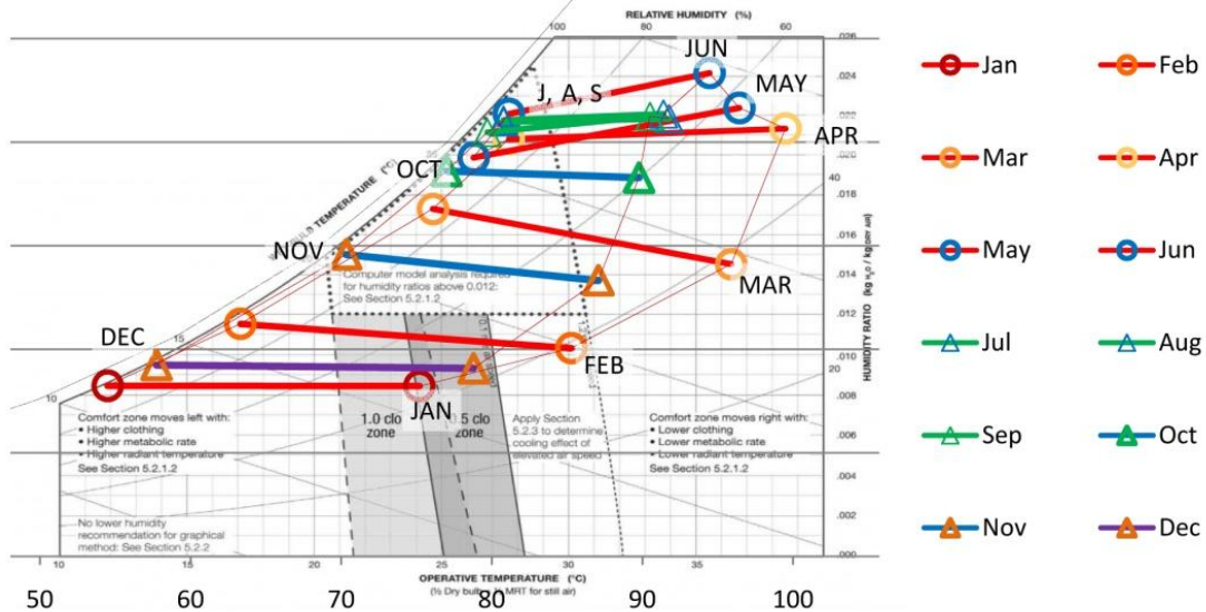
Fig. 2: Calcutta's variations of temperature and moisture superimposed to ASHRAE-55 comfort zone
