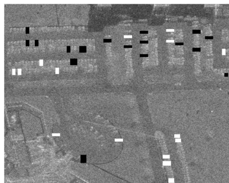
Fig. 8. Empirical ground truth superimposed to the reference image.
