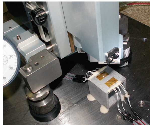
Fig. 3. MTS3000 RESTAN (REsidual STress ANalyzer) system by SINT Technology during a measurement phase on specimen E.
