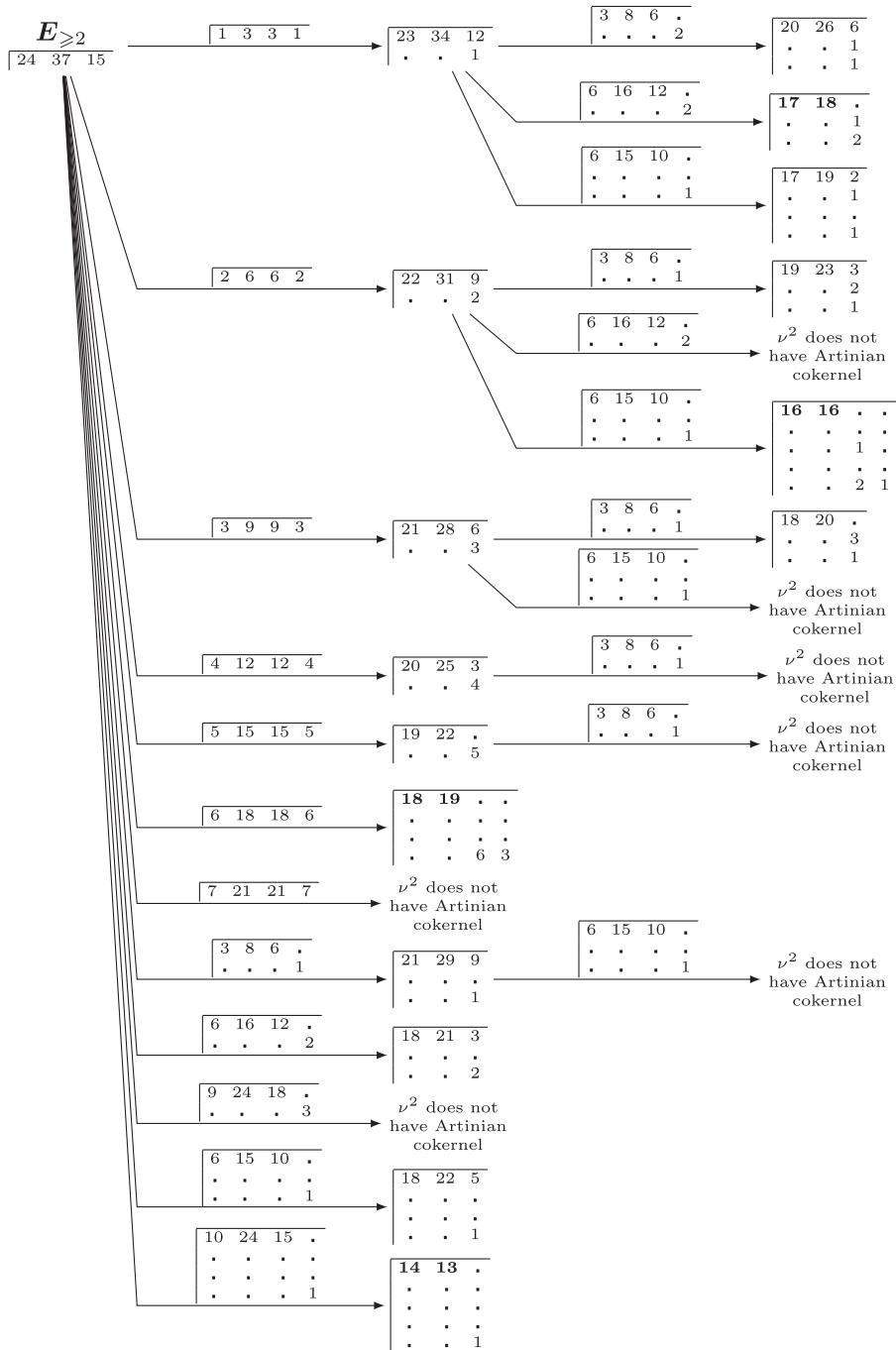
Fig. 1. The set of constant rank matrices that can be produced with our method applied to the truncation E_{\geq 2} = \bigoplus_{t \geq 2} H^0(\mathbb{P}^2(t-1)) the module of global sections of a twist of the tangent bundle E = T_{\mathbb{P}^2}(-1) .
