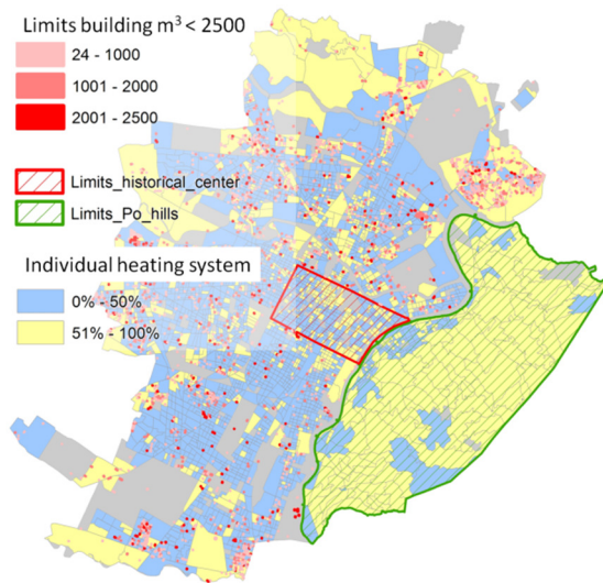
Figure 2a. DH network expansion constraints: individual heating systems (in yellow), Po river and hill (in green), historical centre (in red) and buildings with a volume <math>< 2,500 m^3</math>
