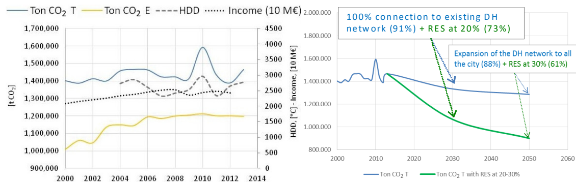
Figure 9a. Thermal and electrical emissions considering HDD and per capita income
