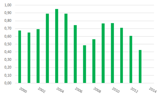
Figure 11b. Energy Security Index for residential sectors: (I1 + I2 + I3 + I4)/4
