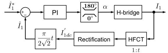
Fig. 5: Control block scheme of the H-bridge.
