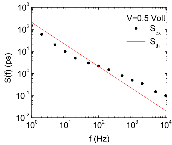
Fig. 8: Relative excess current-noise power spectral density S(f) or the Au/Tc/Al sample of [17] for an applied voltage of 0.5 Volt at room temperature. Symbols refer to experiments, continuous line to theory (see text).
