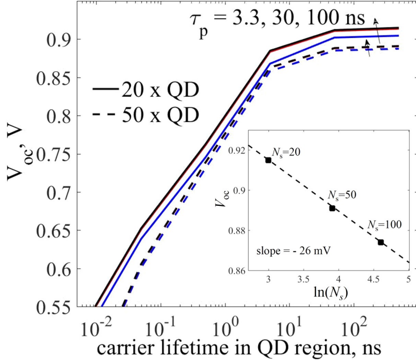
Figure 6: Behavior of V_{oc} for the 20× (solid lines) and 50× (dashed lines) QD cells as a function of the non radiative recombination lifetime in the interdot layers of the QD stack, for different values of hole SRH lifetime in the doped portion of the emitter ( \tau_p ). The insets shows the scaling of V_{oc} with the natural logarithm of the number of QD layers ( N_s ): symbols are results of simulations, the dashed line is the linear fitting with 26 mV slope according to V_{oc} = V_T \ln(J_{sc}/J_0) \propto -V_T \ln(N_s) .
