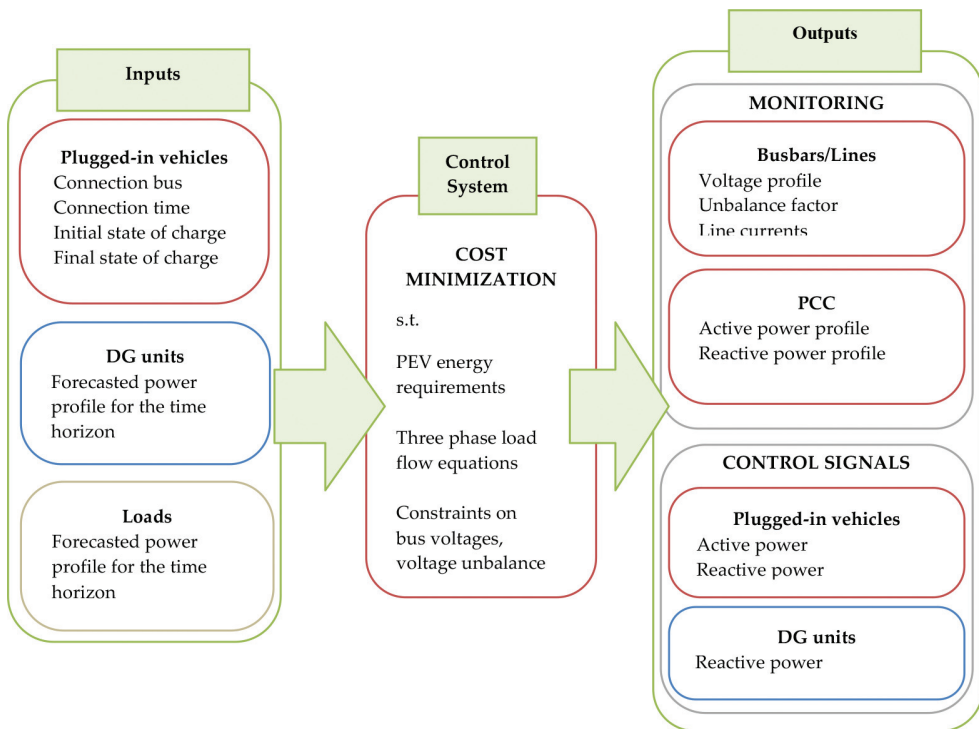
Figure 2. Schematic of the proposed control strategy.
