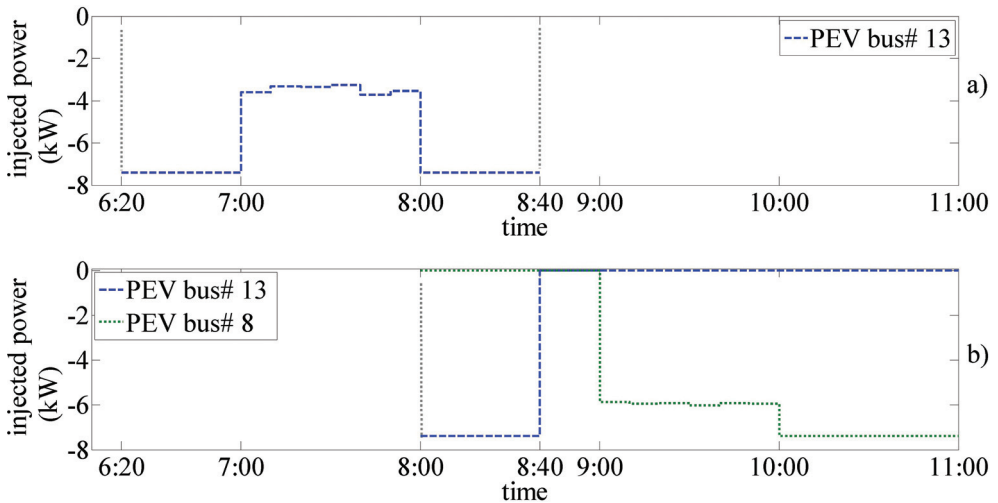
Figure 7. Active power of the PEVs.
