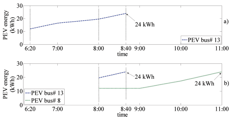
Figure 9. Stored energy of the PEVs during T_1 (a) and T_2 (b).
