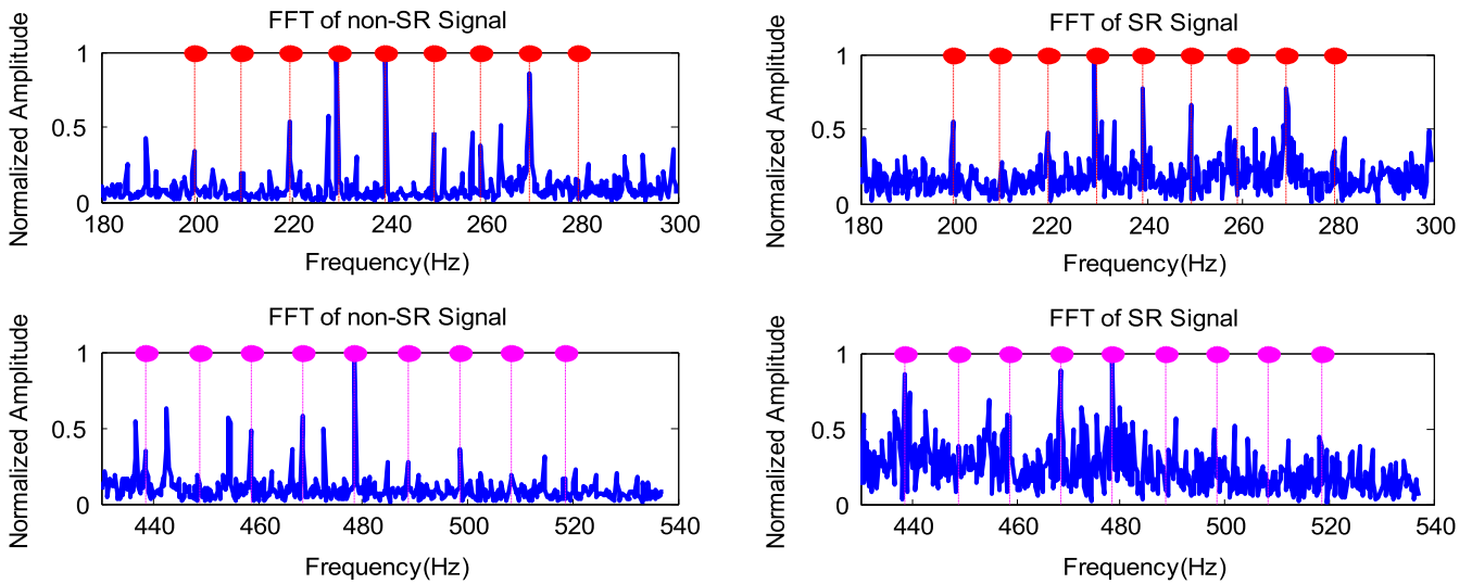
Fig. 9. Non-SR and SR vibration spectrum of a 1800 rpm double stage reduction helical gearbox–chipped tooth case (a) lower meshing frequency range (b) upper meshing frequency range.
