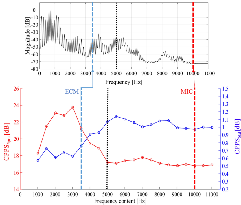
Fig. 7. (Bottom part) - Behavior of CPPS_{5\text{prc}} (red line) and CPPS_{\text{std}} (blue line) vs frequency content of the spectrum. (Upper part) - Spectrum magnitude of the vowel under investigation, acquired with the headworn microphone. Vertical dashed lines correspond to the frequency content of signals acquired with the ECM (blue line) and with the headworn microphone (red line). Vertical dotted black lines helps in reading the graphs.
