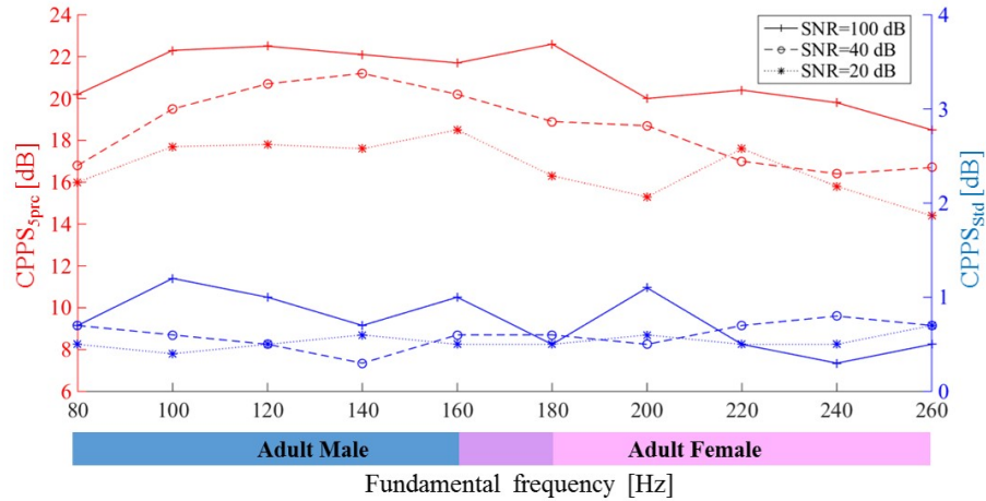
Fig. 5. Behavior of CPPS_{5prc} (red lines) and CPPS_{std} (blue lines) vs fundamental frequency, for three SNR levels (100 dB, 40 dB and 20 dB).
